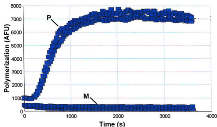
Fluorescence enhancement during pyrene actin polymerization.
