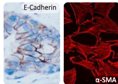
α-SMA
